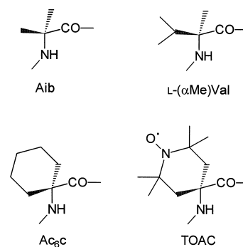
Figure 1. Chemical structures of the C ^{\alpha} -tetrasubstituted \alpha -amino acids Aib, L-( \alpha Me)Val, Ac _6 c, and TOAC.
