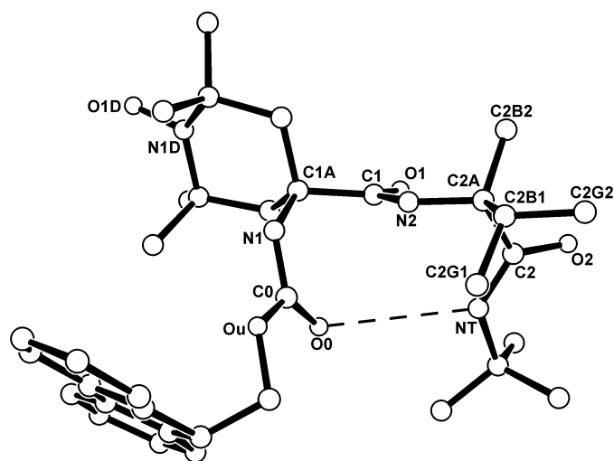
Figure 3. X-ray diffraction structure of Fmoc-TOAC-L-( \alpha Me)Val-NHtBu ( 1 ). The intramolecular C=O...H–N hydrogen bond is represented by a dashed line.
