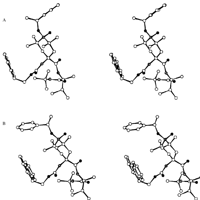
Figure 5. Stereoviews of the minimum energy structures of the diastereomeric intermediates IV (Scheme 1) between Fmoc-TOAC-L-( \alpha Me)Val-NHtBu ( 1 ) and A) ( S )-1-phenylethanol and B) ( R )-1-phenylethanol, with addition of the alcohol on the TOAC ring side close to the Fmoc group.
