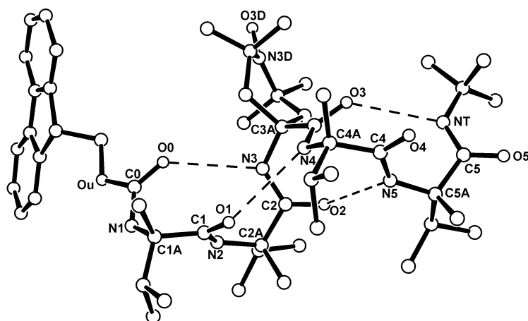
Figure 4. X-ray diffraction structure of Fmoc-[L-( \alpha Me)Val] 2 -TOAC-[L-( \alpha Me)Val] 2 -NHtBu ( 15 ). The intramolecular C=O...H–N hydrogen bonds are represented by dashed lines.
