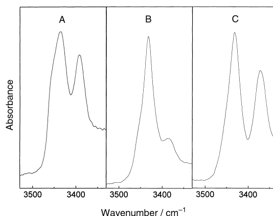
Figure 2. FTIR absorption spectra in the N–H stretching region (3500–3350 cm -1 region) of A) Fmoc-TOAC-L-( \alpha Me)Val-NHtBu ( 1 ), B) Fmoc-TOAC-L-Val-NHtBu ( 12 ), and C) Fmoc-L-( \alpha Me)Val-TOAC-NHtBu ( 14 ) in CDCl 3 solution (conc. 1 mM).
